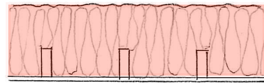
Ceiling to roof space 400mm fibre insulation
