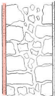
External wall insulation e.g. cork lime render
