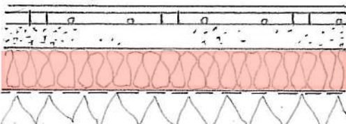
Excavated & new ground floor slab with underfloor heating & floor finish
