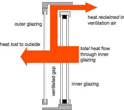
heat flows through the Supply Air Window
