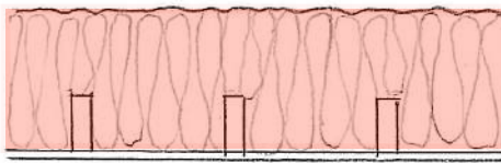
Ceiling to roof space 400mm fibre insulation
