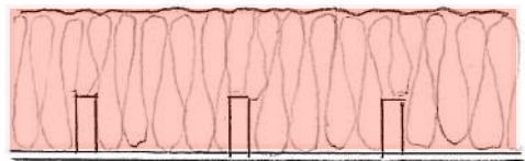
Ceiling to roof space 400mm fibre insulation
