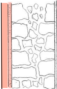
External wall insulation e.g. cork lime render
