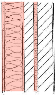
South wing wall external insulation render + cavity fill
